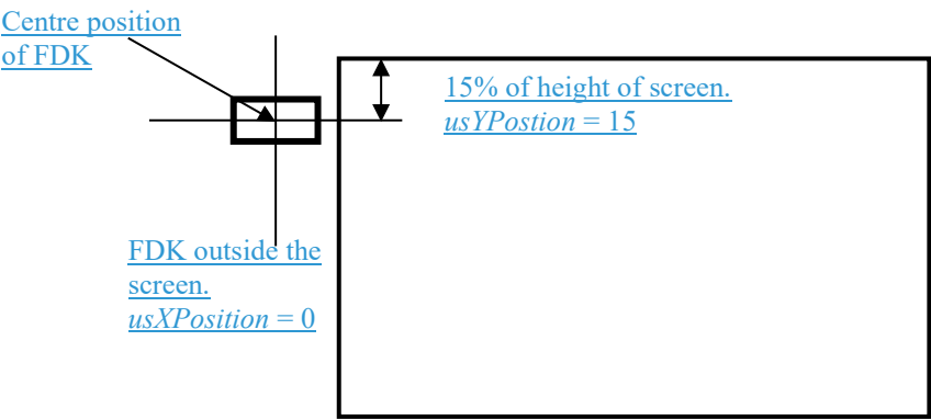
Diagram: Shows how usXPosition and usYPosition are set.
